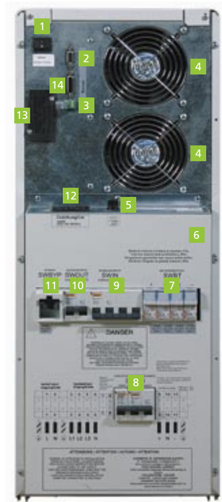
Rear panel PWP 650-800-1000
